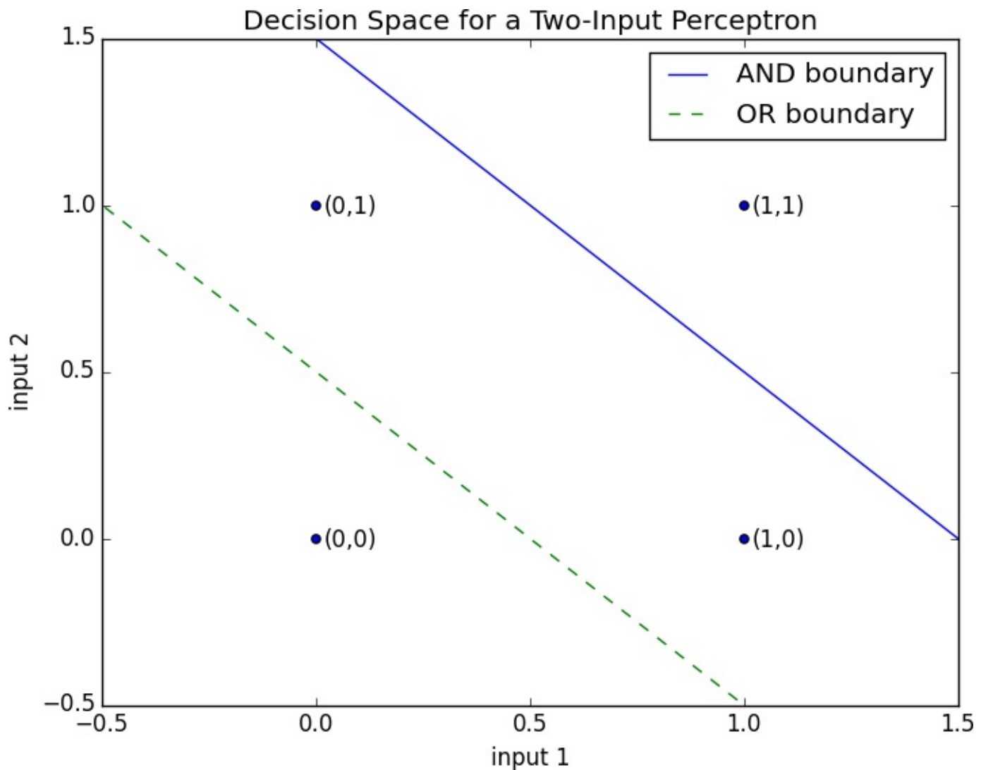
Figure 18-1. Decision space for a two-input perceptron
