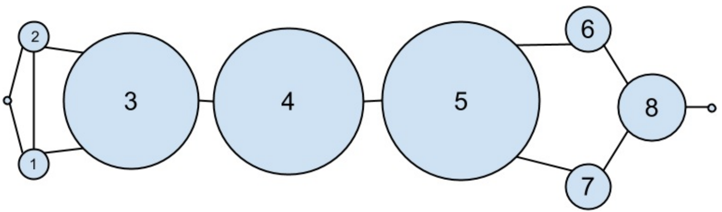
Figure 22-2. The DataSciencecenter network sized by betweenness centrality
