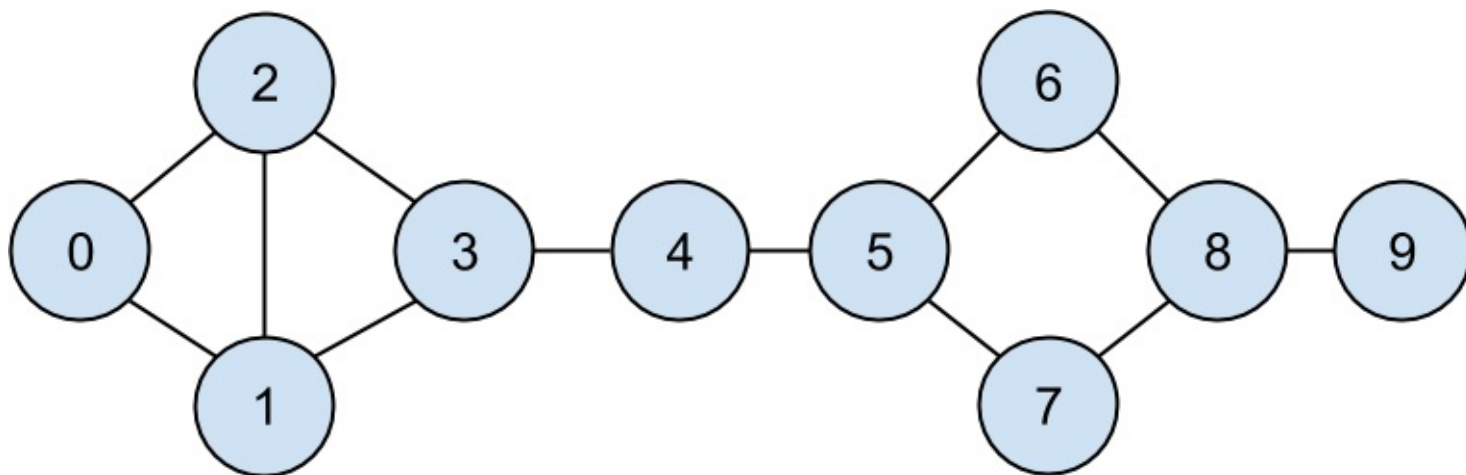
Figure 1-1. The DataSciencecenter network
