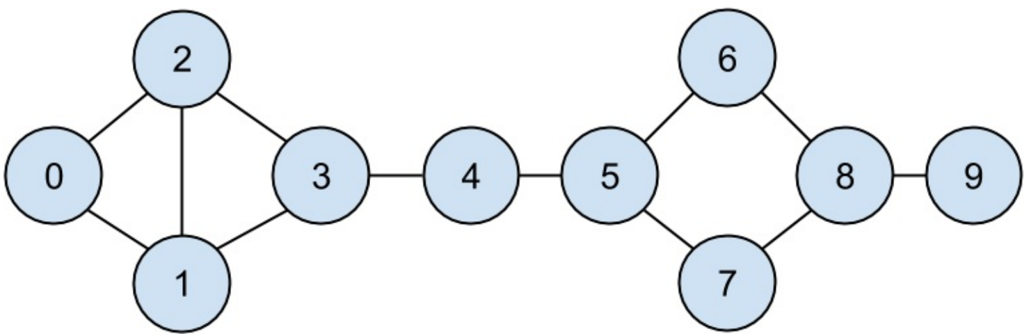
Figure 22-1. The DataSciencecenter network
