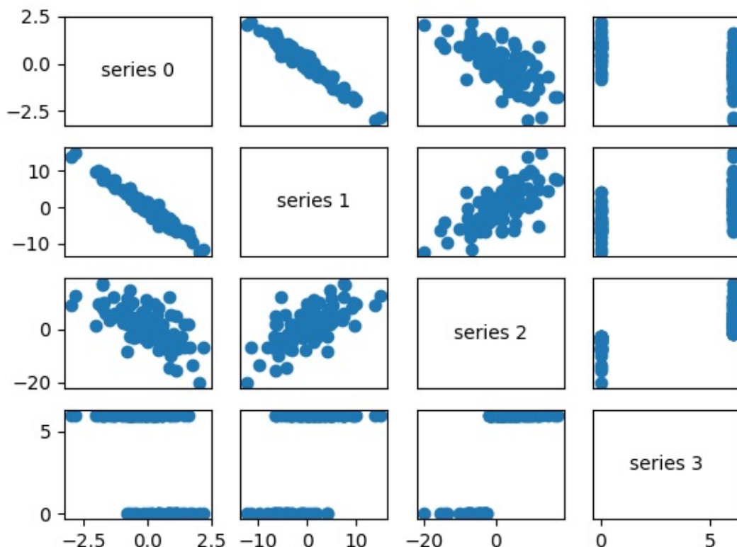
Figure 10-4. Scatterplot matrix
