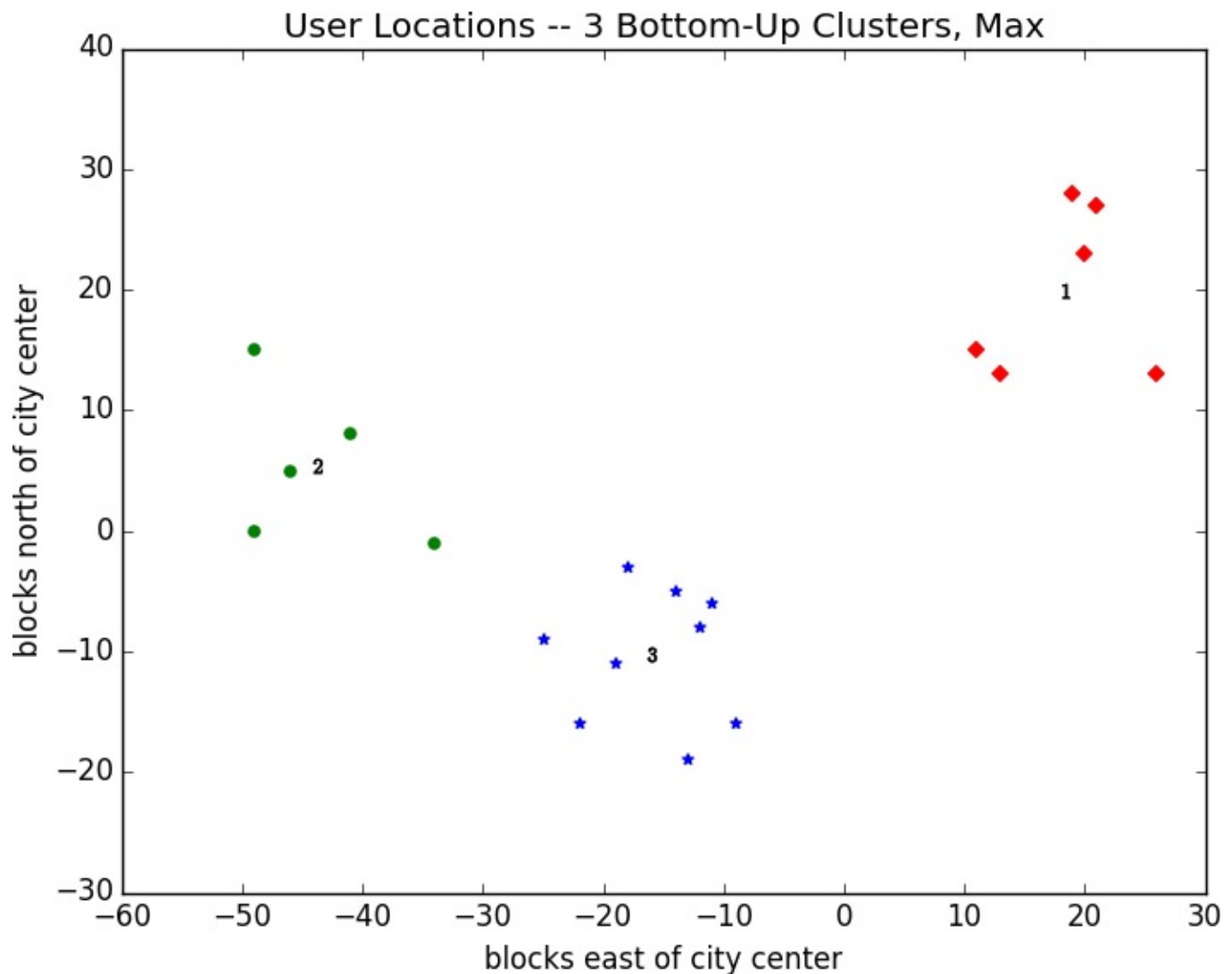
Figure 20-7. Three bottom-up clusters using max distance
