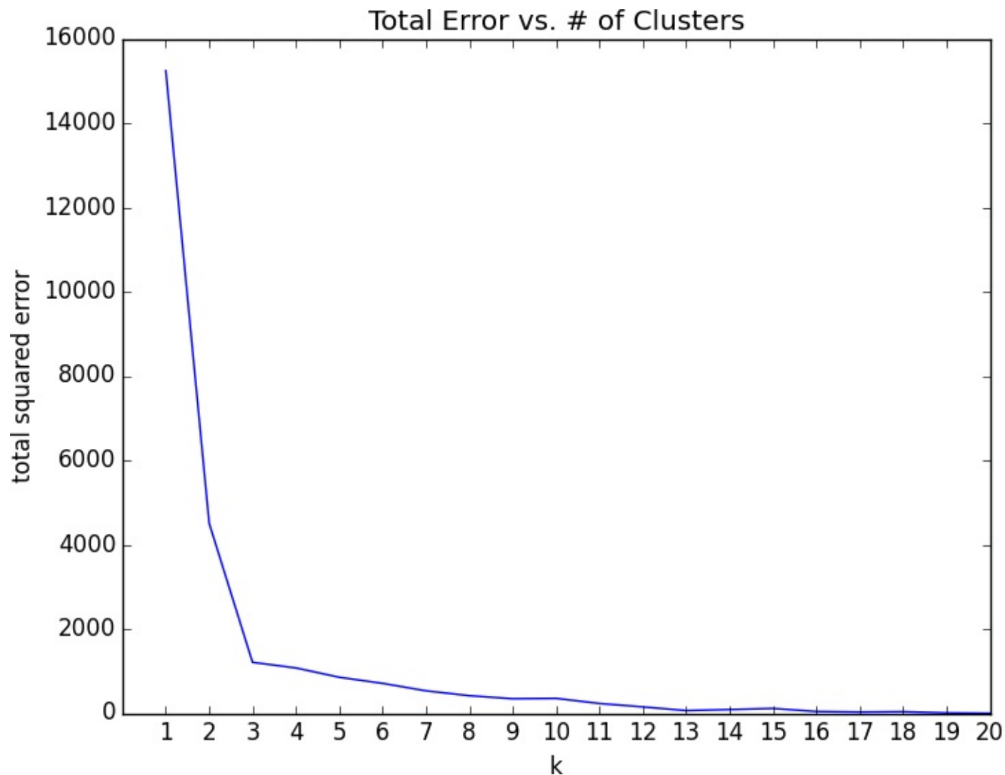
Figure 20-4. Choosing a k
