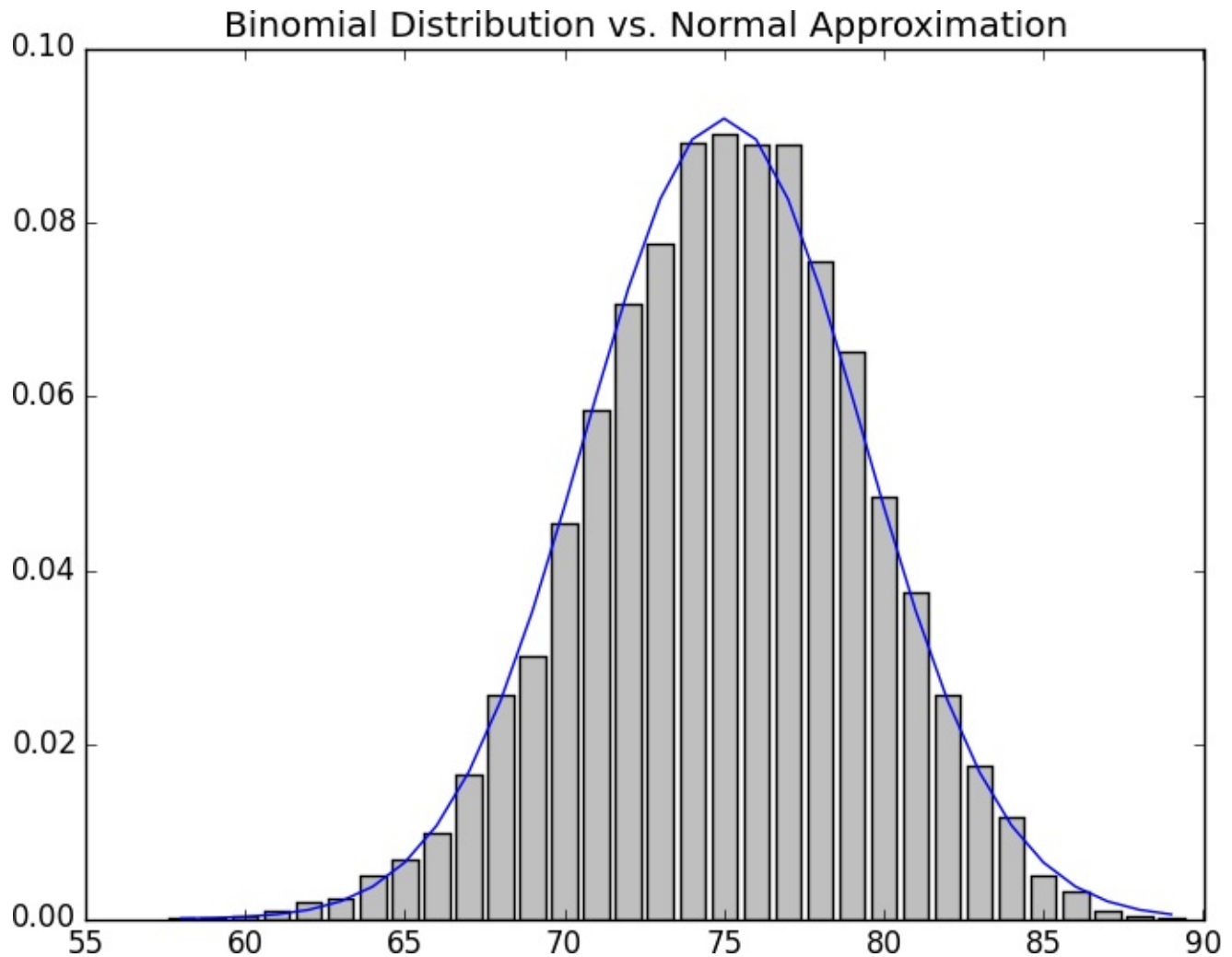
Figure 6-4. The output from binomial_histogram
