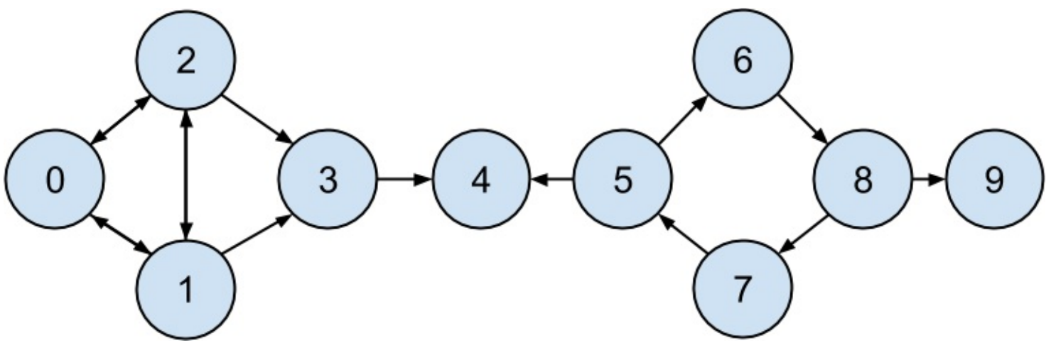
Figure 22-5. The DataSciencecenter network of endorsements
