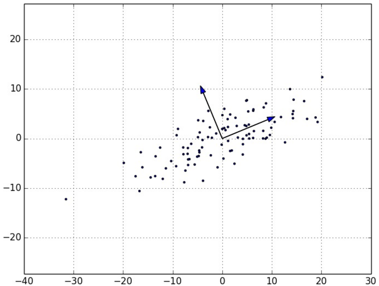
Figure 10-10. First two principal components
