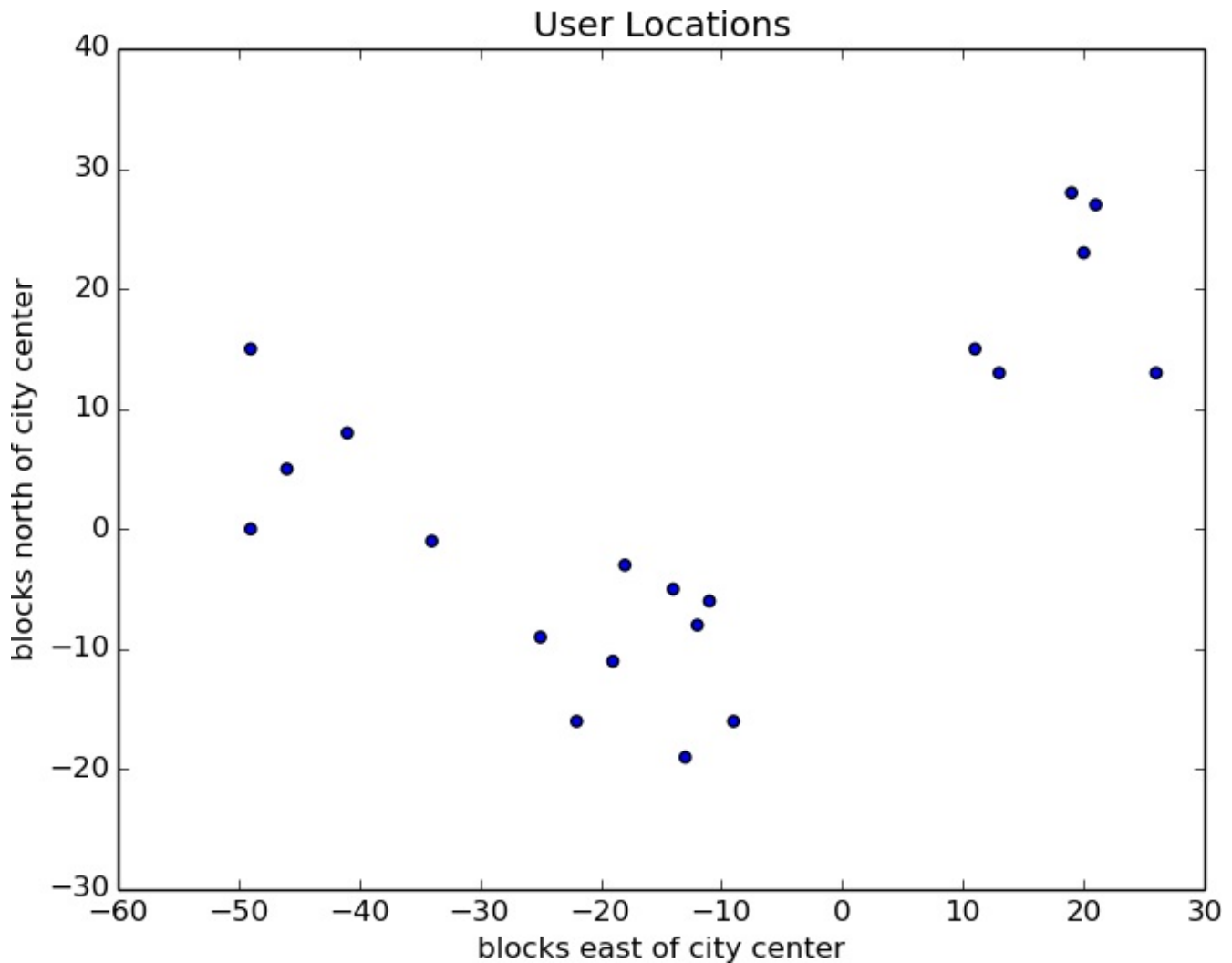
Figure 20-1. The locations of your hometown users
