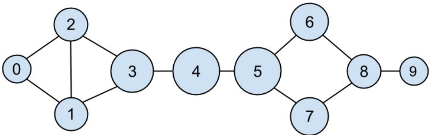
Figure 22-3. The DataSciencecenter network sized by closeness centrality
