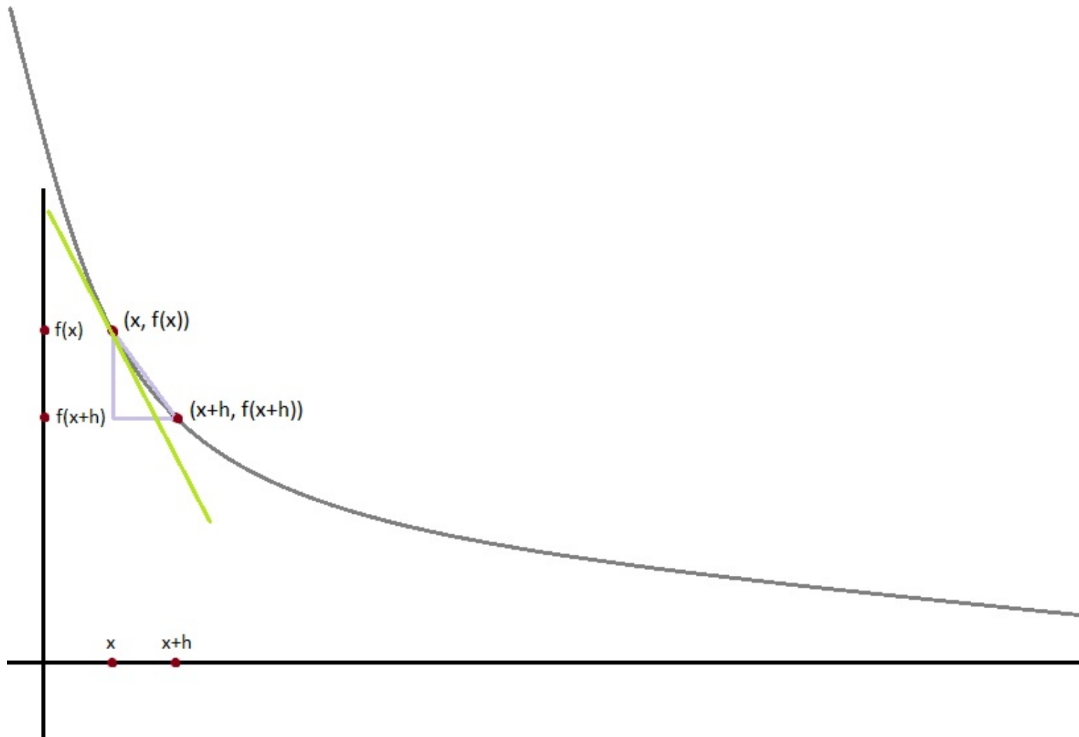
Figure 8-2. Approximating a derivative with a difference quotient
