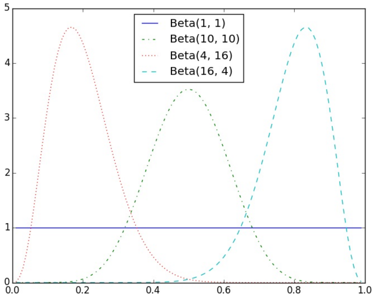
Figure 7-1. Example Beta distributions
