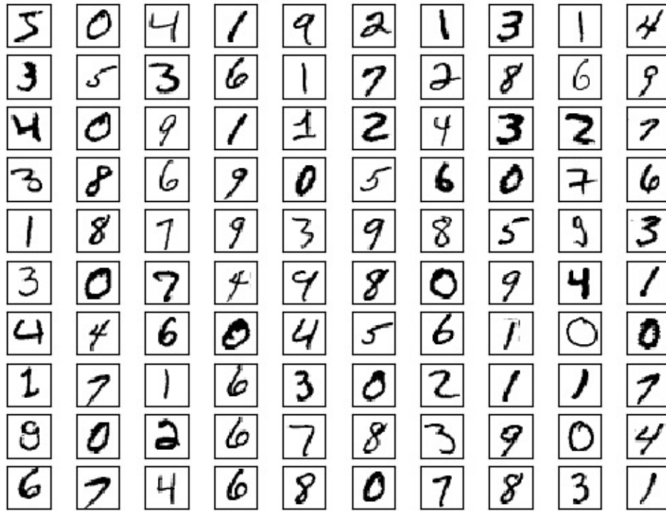
Figure 19-1. MNIST images
