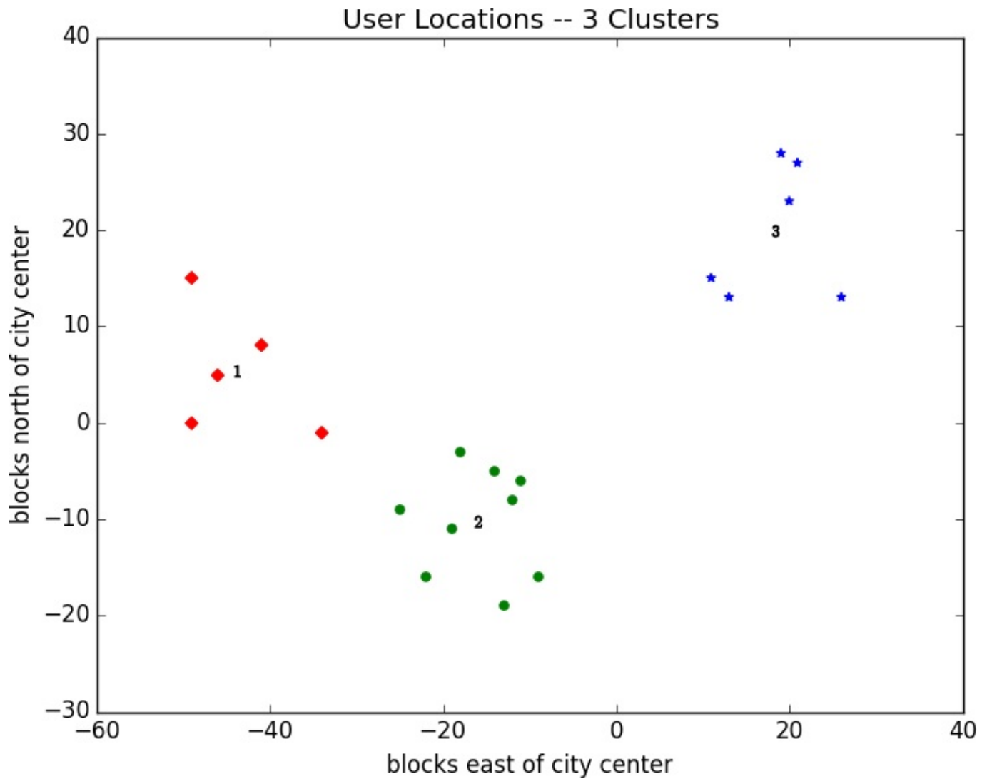
Figure 20-2. User locations grouped into three clusters
