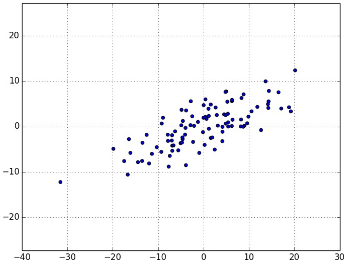
Figure 10-7. Data after de-meaning
