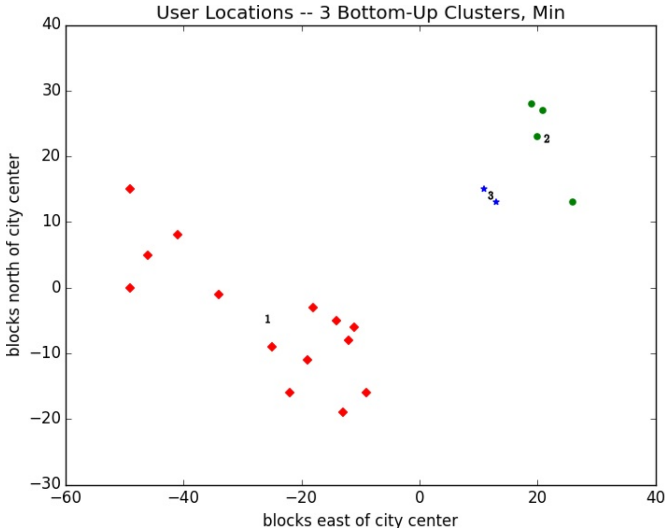
Figure 20-6. Three bottom-up clusters using min distance
