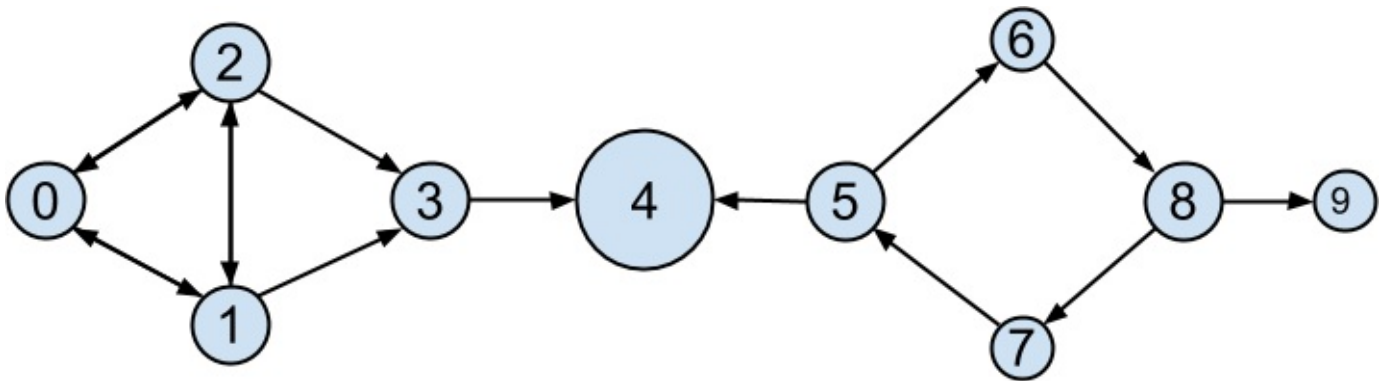
Figure 22-6. The DataSciencecenter network sized by PageRank
