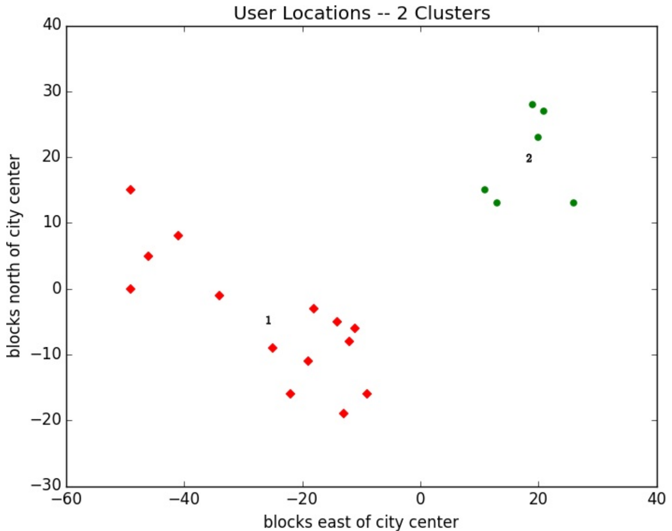
Figure 20-3. User locations grouped into two clusters
