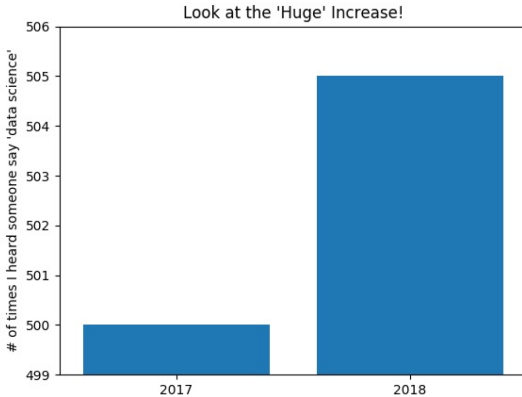
Figure 3-4. A chart with a misleading y-axis
