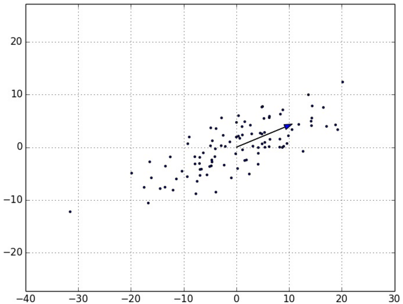
Figure 10-8. First principal component
