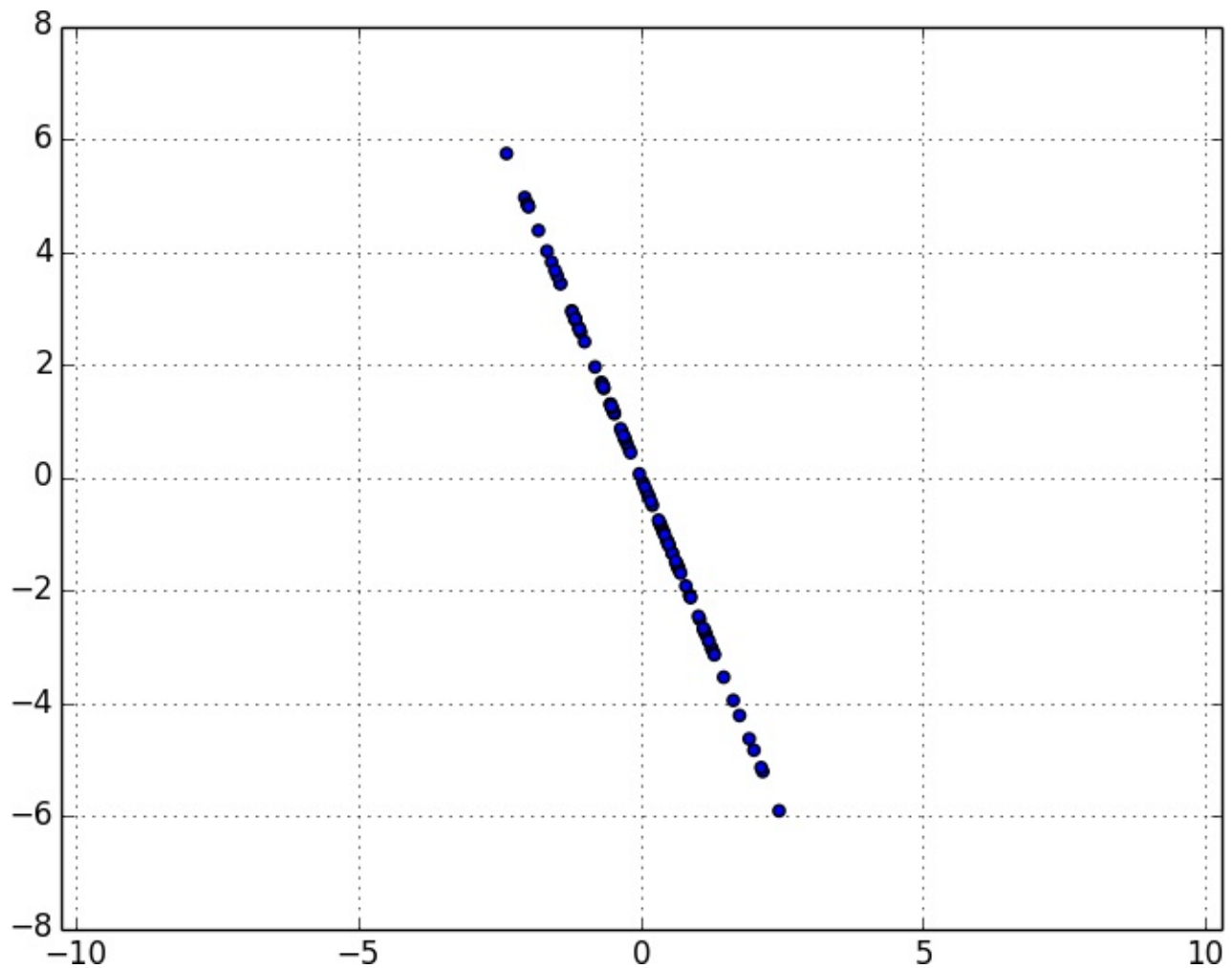
Figure 10-9. Data after removing the first principal component
