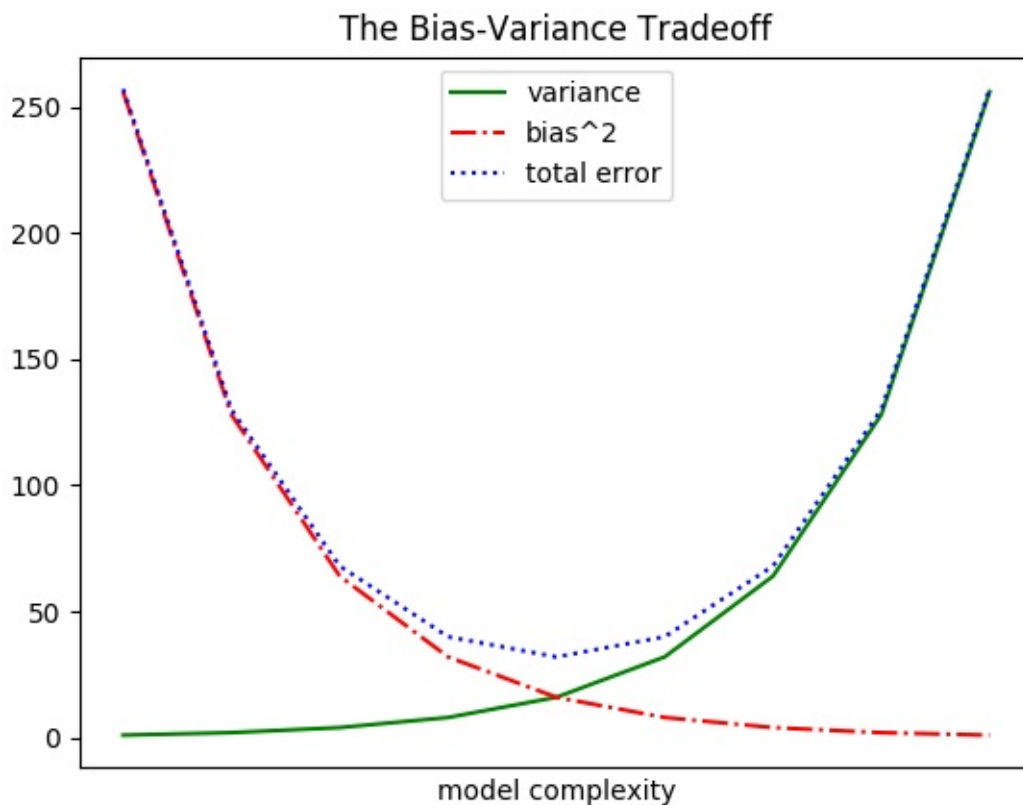
Figure 3-6. Several line charts with a legend
