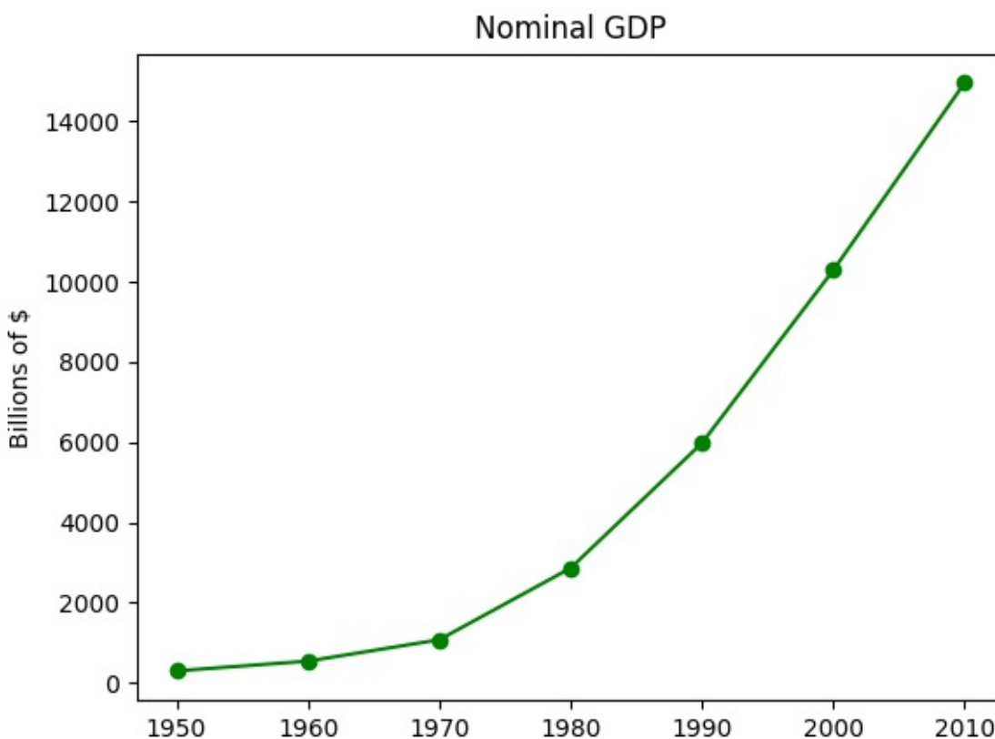
Figure 3-1. A simple line chart
