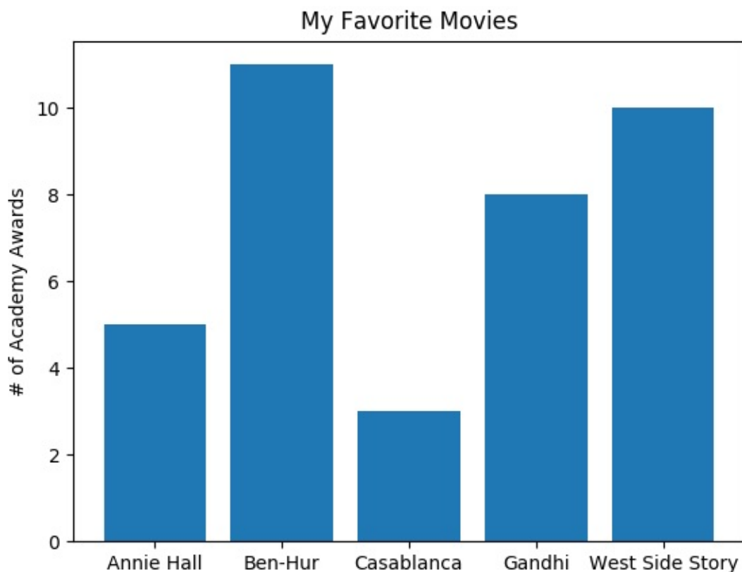
Figure 3-2. A simple bar chart
