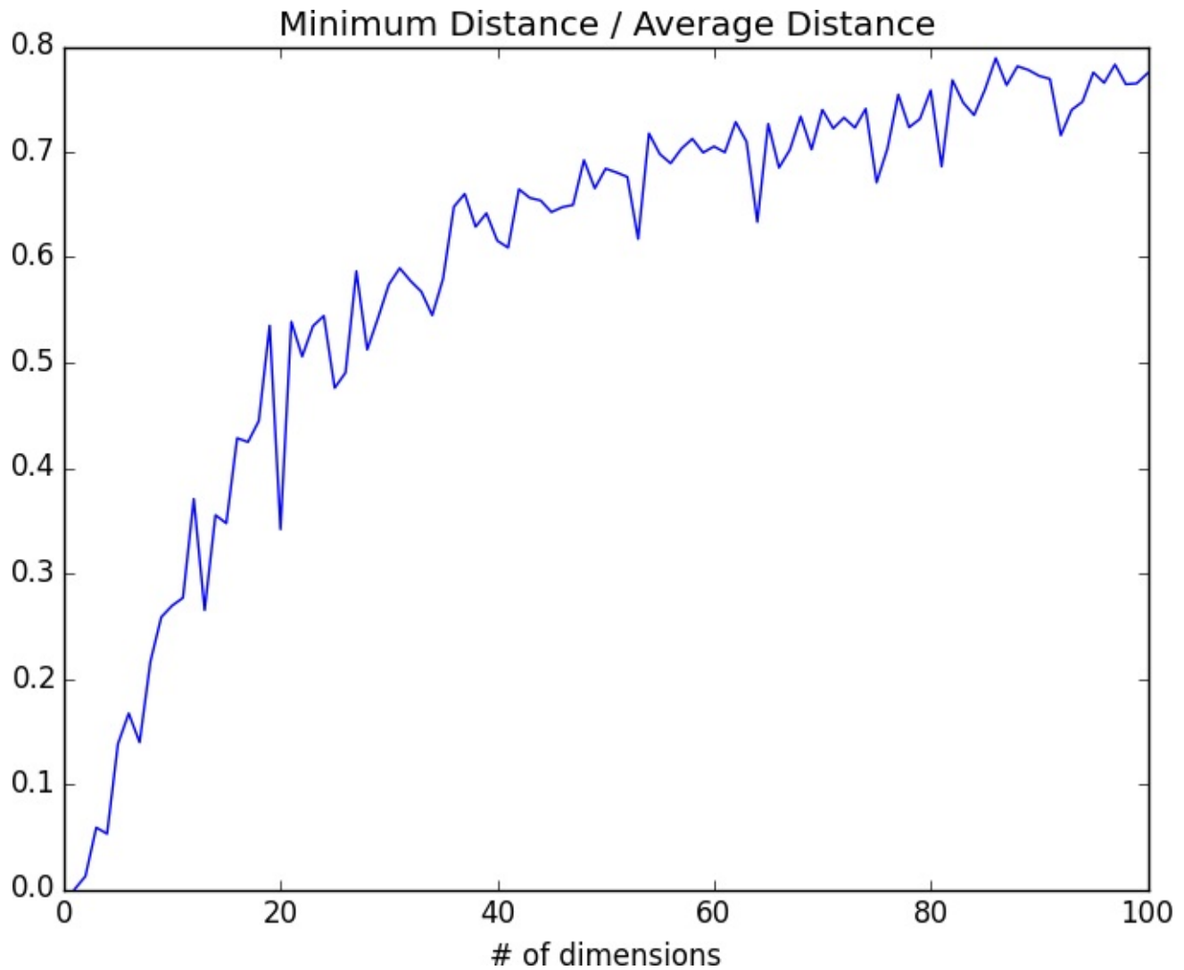
Figure 12-3. The curse of dimensionality again
