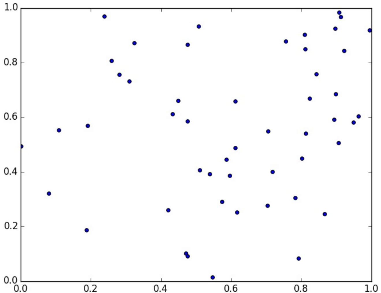
Figure 12-5. Fifty random points in two dimensions
