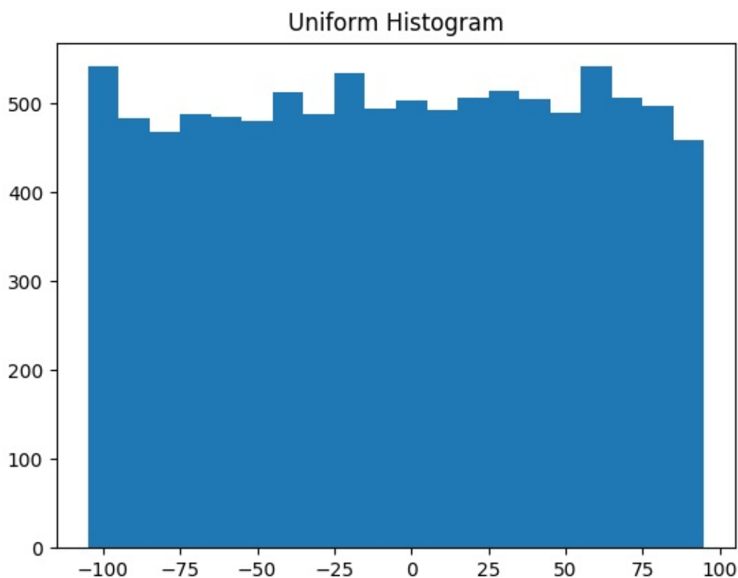
Figure 10-1. Histogram of uniform
