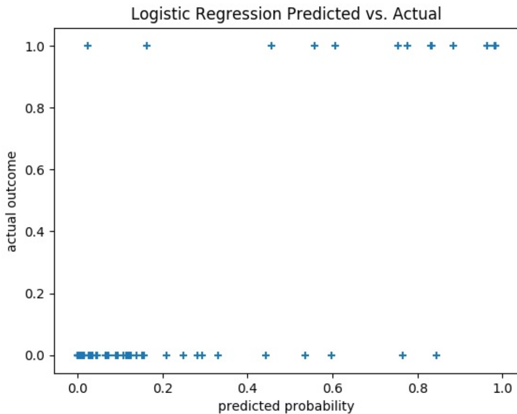
Figure 16-4. Logistic regression predicted versus actual
