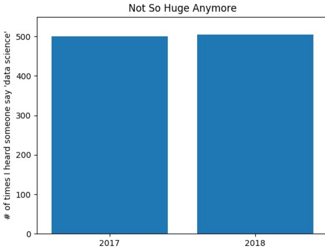
Figure 3-5. The same chart with a nonmisleading y-axis
