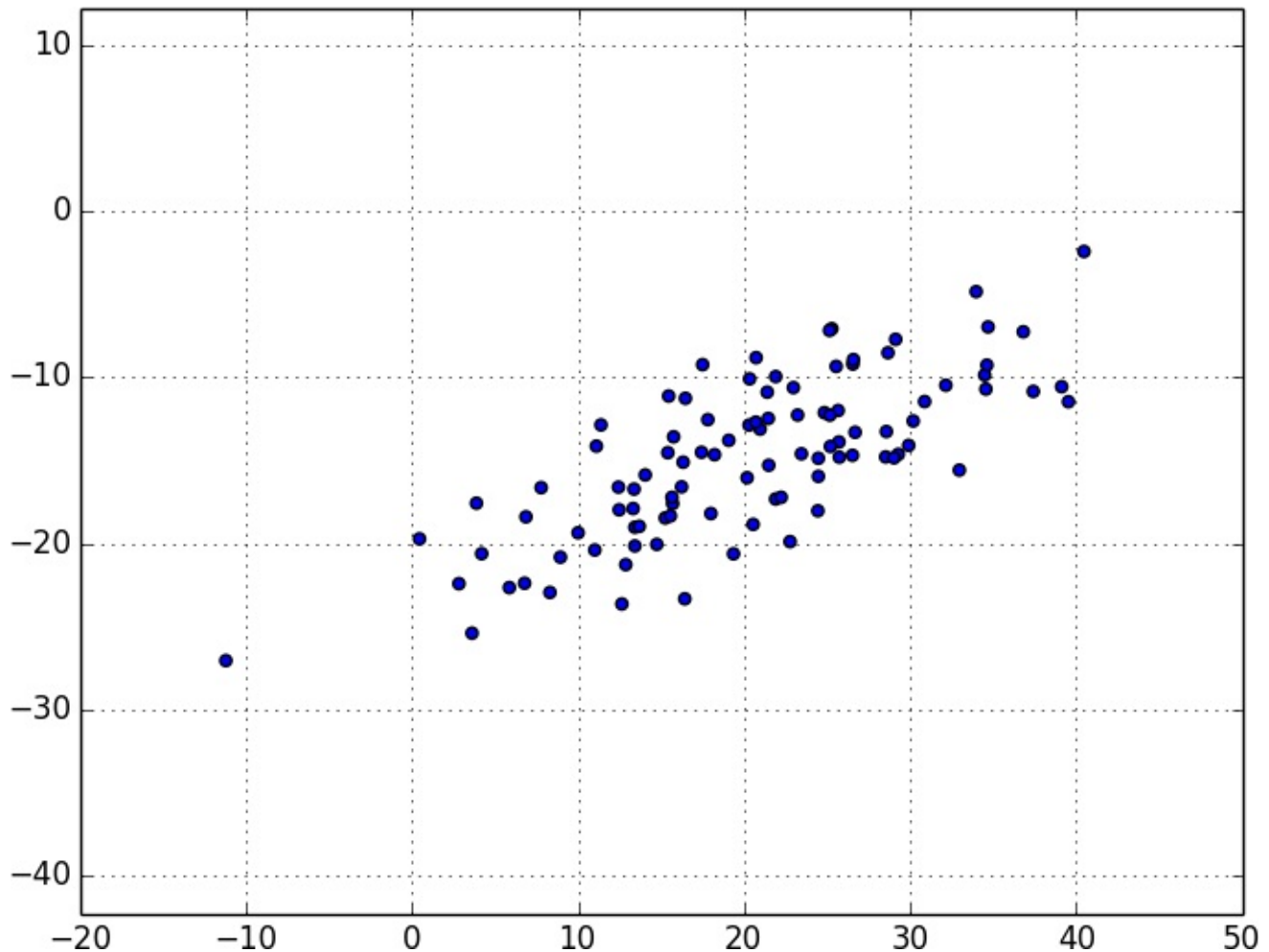
Figure 10-6. Data with the “wrong” axes
