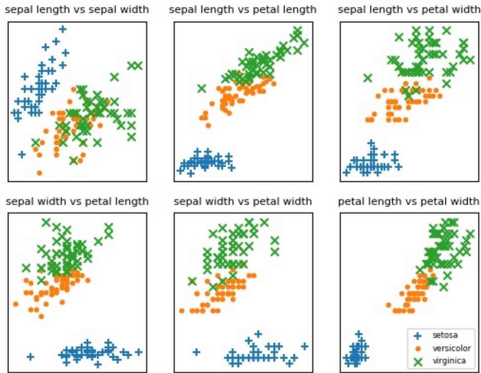
Figure 12-1. Iris scatterplots
