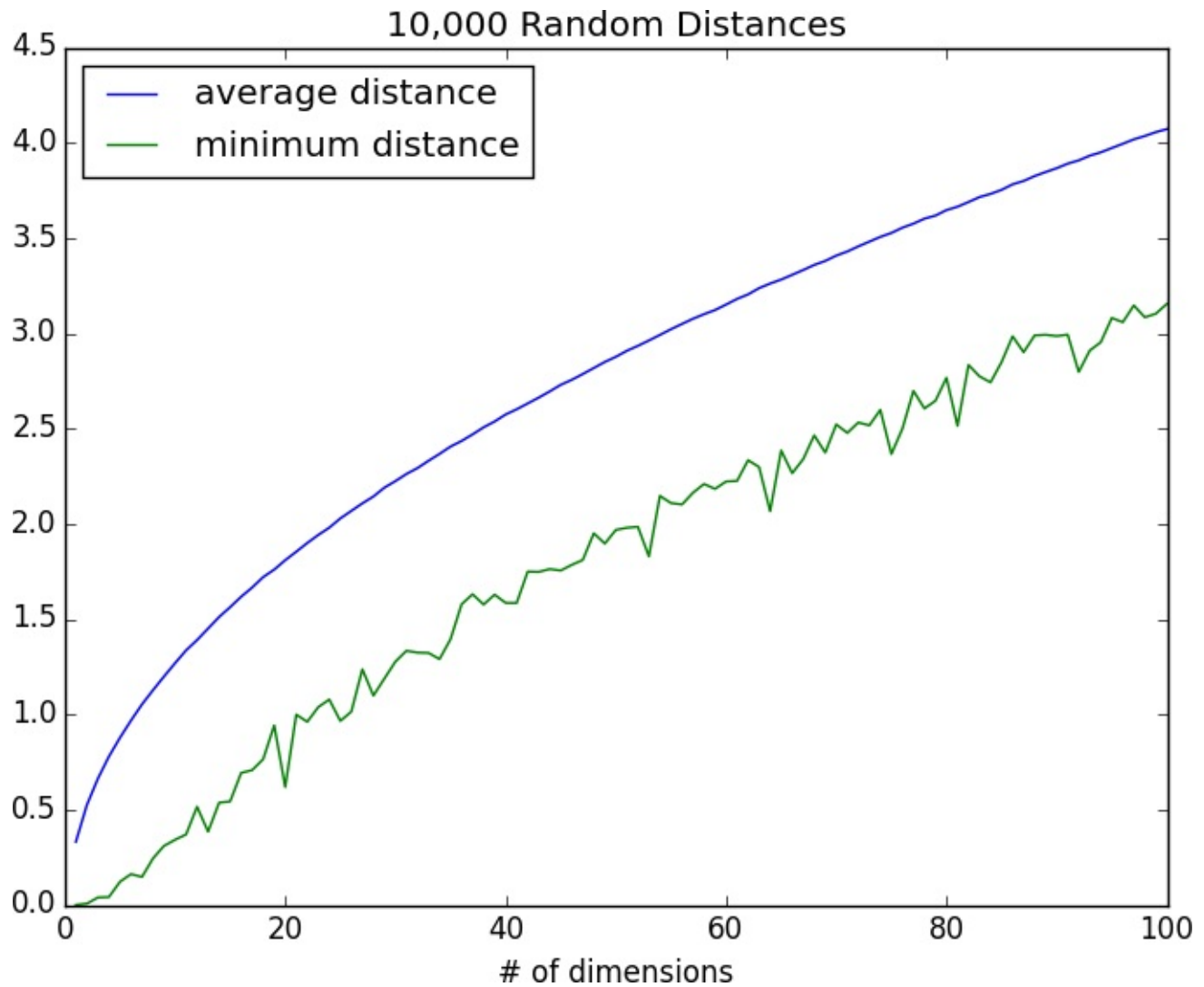
Figure 12-2. The curse of dimensionality
