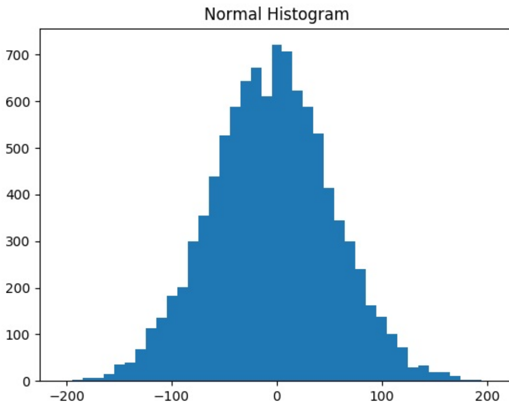
Figure 10-2. Histogram of normal
